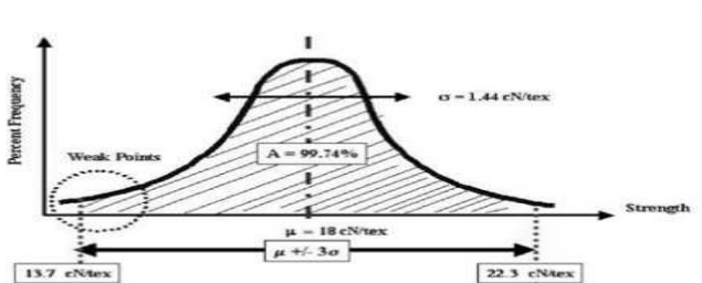
Figure 7.11. Distribution of Yarn Strength
