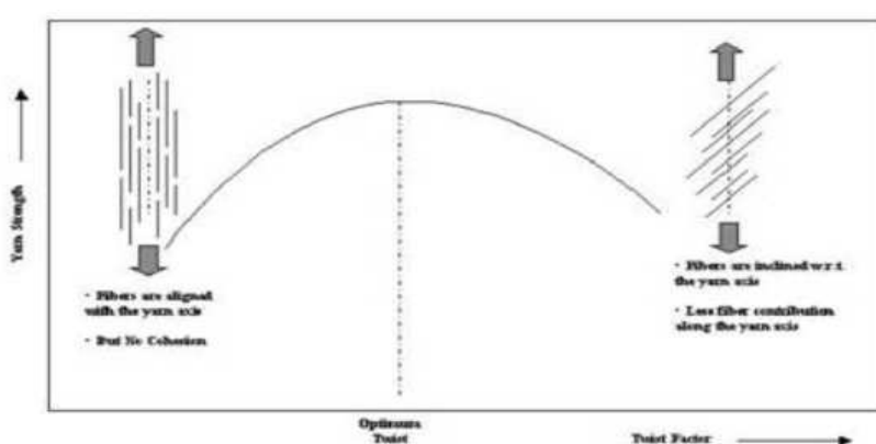
Figure 7.7. Effect of Twist on Spun-Yarn Strength
