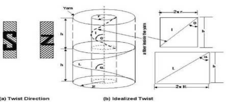
Figure 7.6. Twist Direction and Twist Level of Idealized Yarn Geometry
