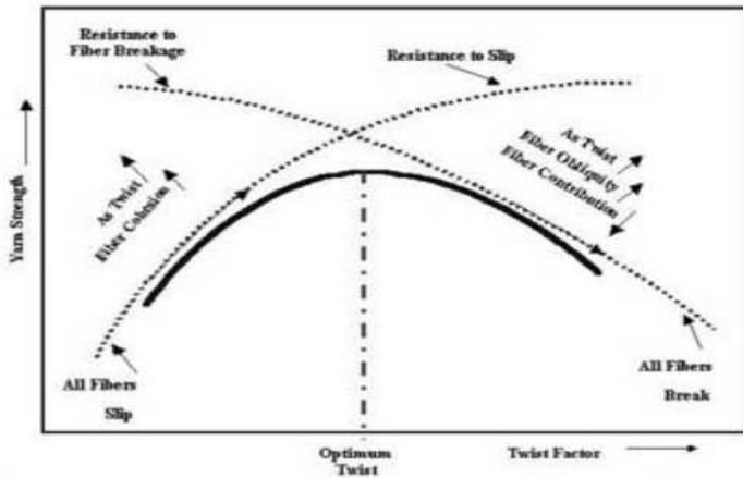
Figure 7.8. Interpretation of Strength-Twist Relationship
