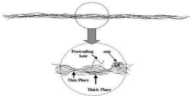
Figure 7.12. Different Imperfections in a Spun Yarn
