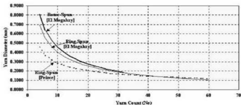
Figure 7.9. Relationships Between Yarn Diameter and Yarn Count
